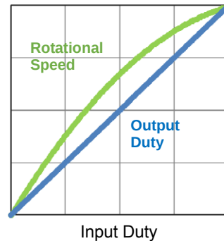
Figure 22. Properties Curve of Input PWM Duty vs Rotational Speed
