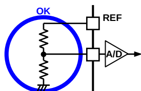
Resistor Divider
