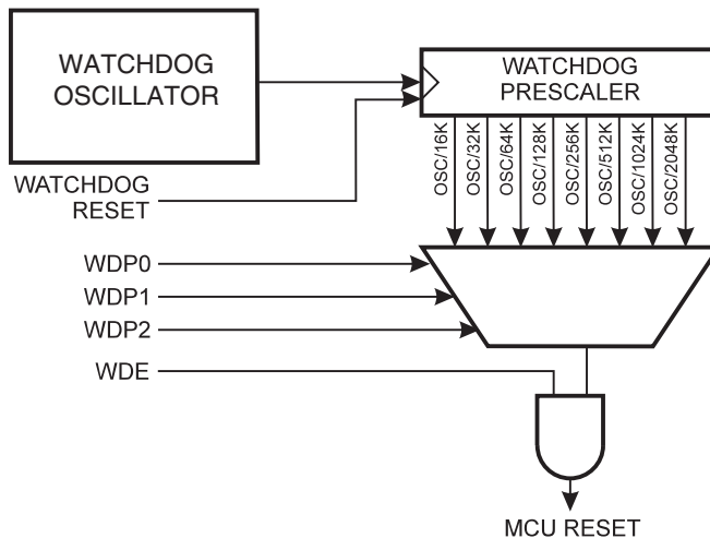
Figure 20. Watchdog Timer
